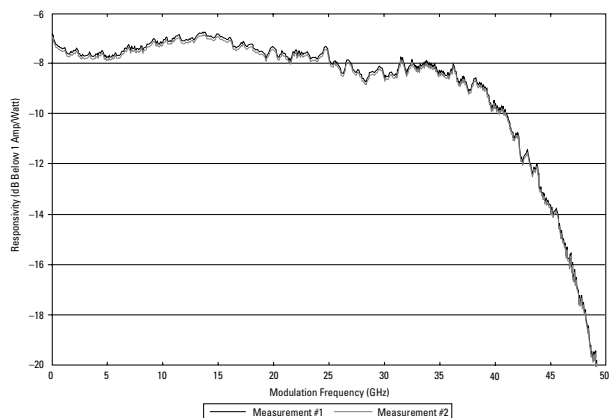
Figure 6. Typical short-term measurement repeatability; the two traces overlay almost exactly.
