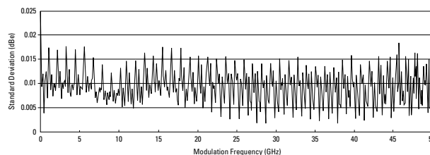
Figure 9. Typical sweep-to-sweep repeatability.
