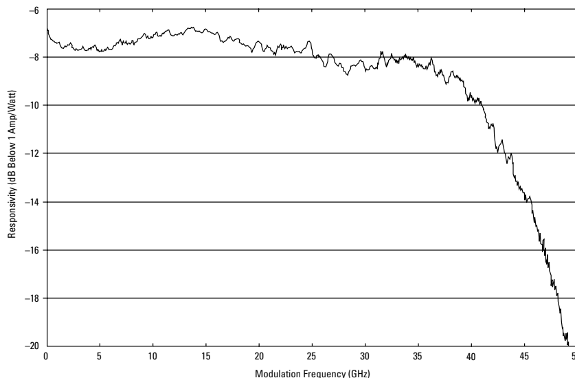
Figure 4. Typical measured data of an O/E converter displayed in Microsoft Excel format.
